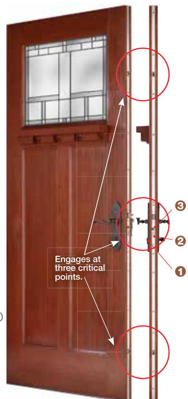
Heirloom Venture Millennium Backplates: Wide / Narrow; Locking: Active / Inactive (Not Shown)
