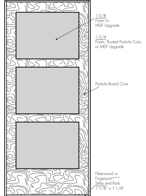
SOLID CORE CONSTRUCTION
