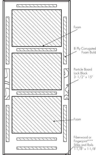
HOLLOW CORE CONSTRUCTION
